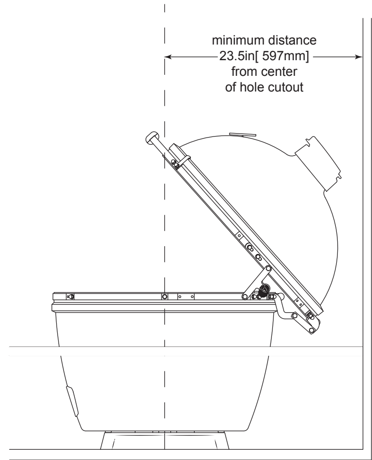
REAR WALL DISTANCE FROM CENTER provides enough clearance for dome when fully opened
